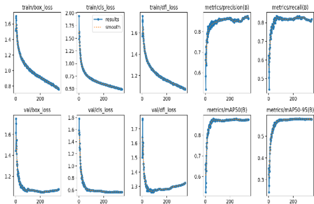
Figure 3. YOLOv11n Model Training Results
