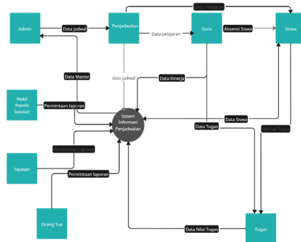
Gambar 2. Data Flow Diagram (DFD)
